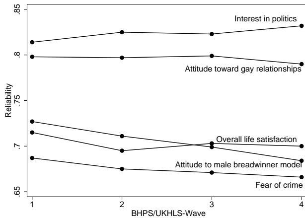
Figure 3. Comparison of reliability estimates: Standard indicator and four attitude items in the BHPS/UKLS. Estimates from Table C1 in the appendix.
