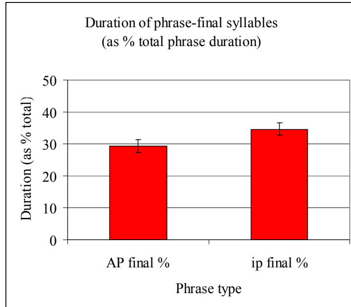
Figure 98. Relative duration of AP-final syllables compared to that of ip-final syllables. Error bars indicate standard error.
