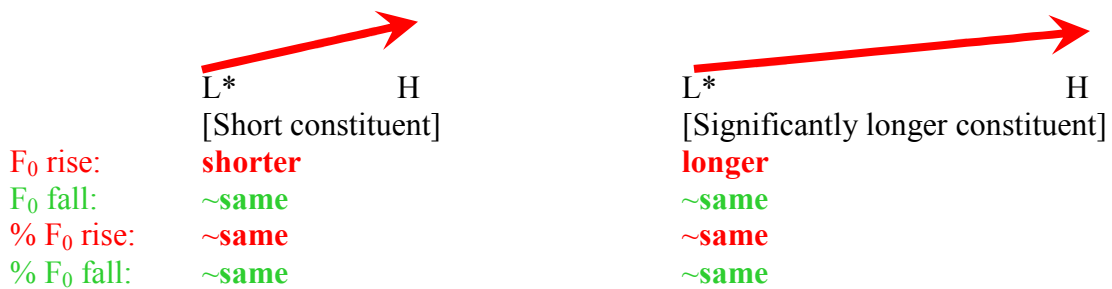
Figure 121. Predicted properties of smooth rises ( L^*\dots Ha ).
