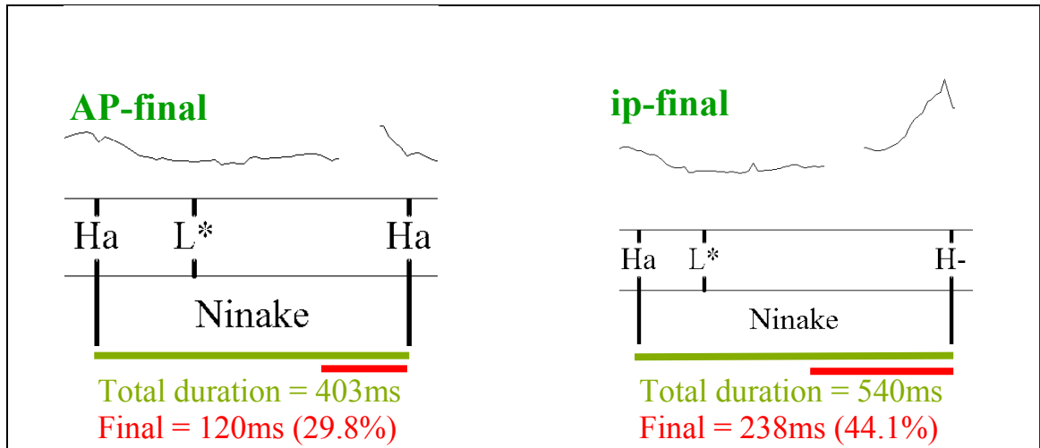
Figure 97. Measuring within speaker, the duration of the final syllable [ke] relative to the whole word [ninake] ‘Nina-ACC’ is longer ip-finally (right) than AP-finally (left) in otherwise identical sentences [paired t(8) = 3.05 , p = .02 ].
