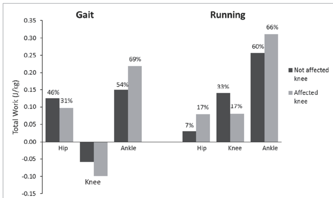
Figure 1: Contribution of the hip, knee and ankle joints to the absorbed and generated energy during stance phase of level walking and running.
