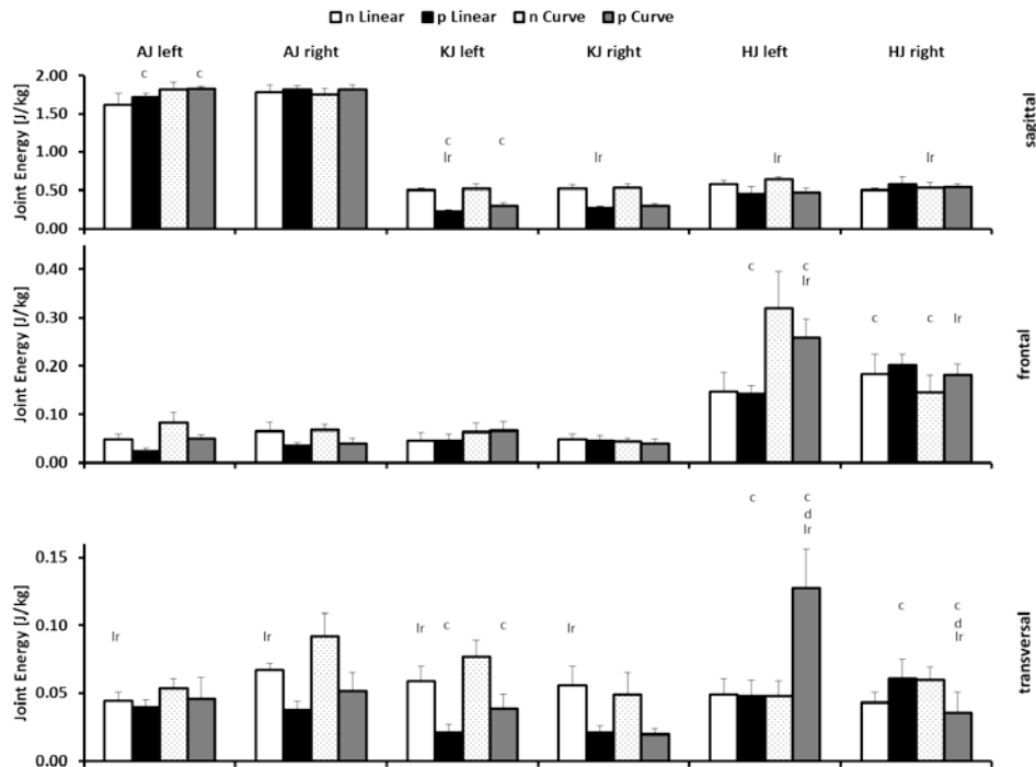
Figure 1: Energy absorption (n) and generation (p) of ankle joint (AJ), knee joint (KJ) and hip joint (HJ) for curve and linear sprinting in the sagittal, frontal and transversal plane.
