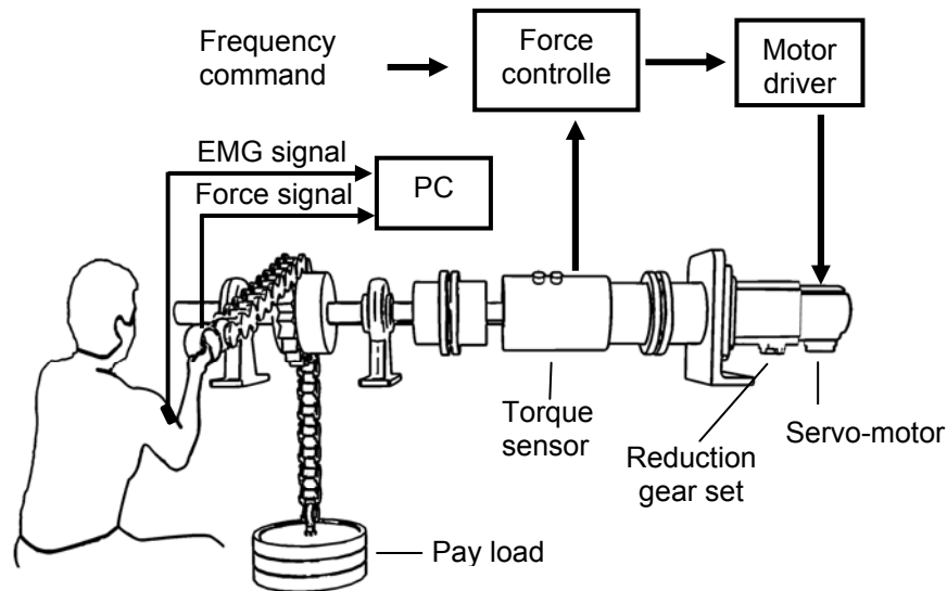
Figure 1: Schematic of the vibratory stimulation system [VSTS].
