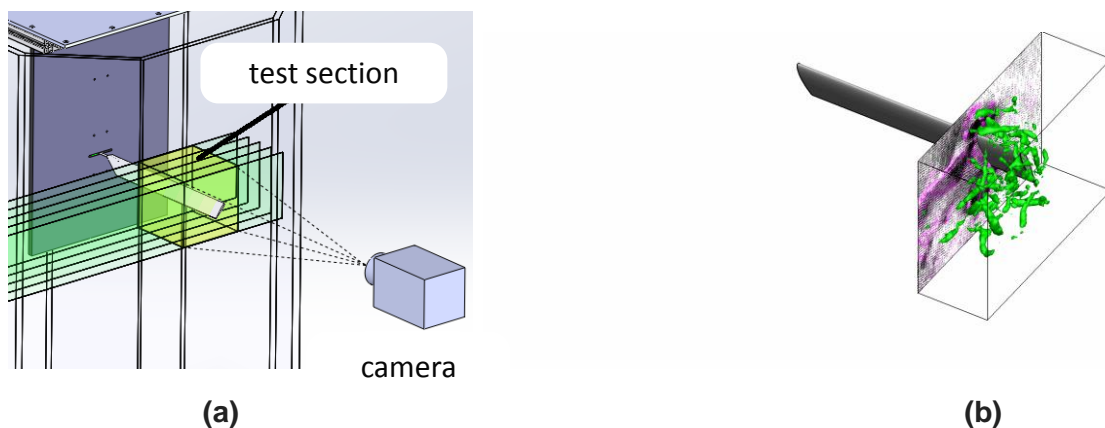
(a) Acquisition of the flow around a flapping wing; (b) \lambda_2 criteria, pressure and velocity measurements from TR PIV.
