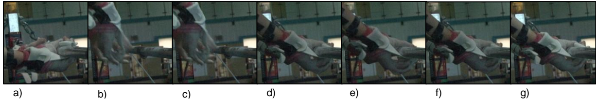
Figure 2. Images of the hand at release using varying methods of release identification during a Takchev; a) J_{FZ} , b) J_{FY} , c) J_{FR} , d) GR_{1\%} , e) GR_{10\%} , f) HS , g) HS_{-1} .
