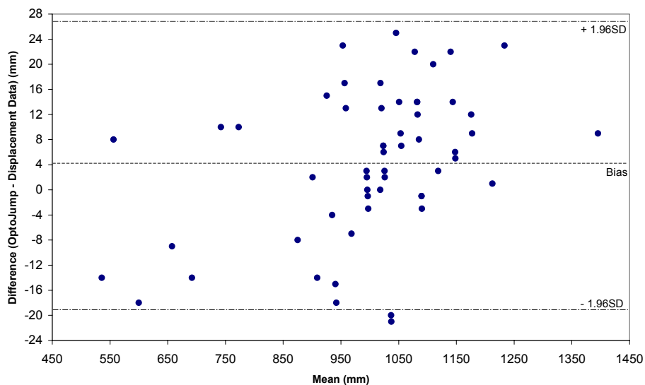
Figure 1 - A Bland-Altman plot with bias line and random error lines forming the 95% limits of agreement.
